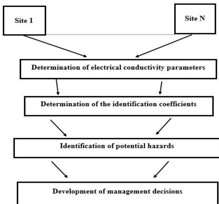
Fig. 1. Block diagram of the author's approach to the prevention of emergencies related to the ingress of pollutants into water or soil.
