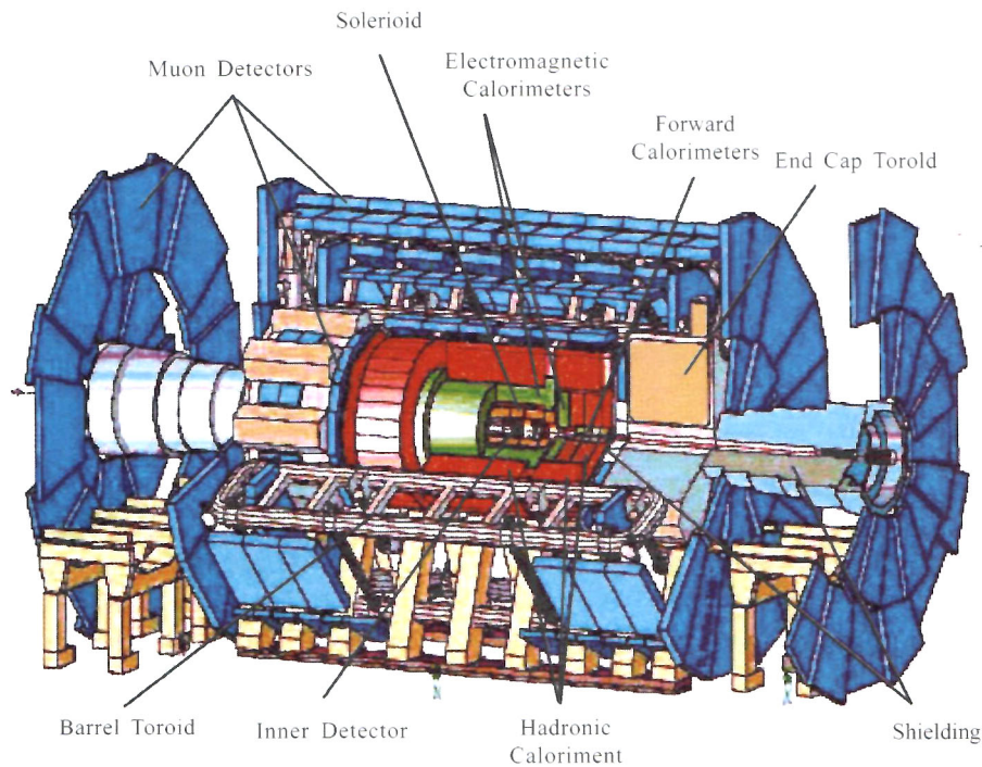
Fig. 1. The ATLAS detector, from [1].
