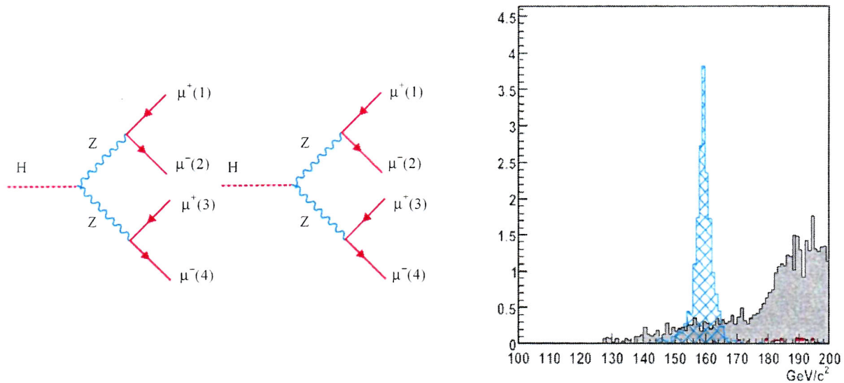
Fig. 2. The identity effects in the Higgs decay H \rightarrow 4\mu (left) Fully reconstructed SM Higgs boson with mass 160 \text{ GeV}/c^2 via its decay H \rightarrow 4\mu . (right).
