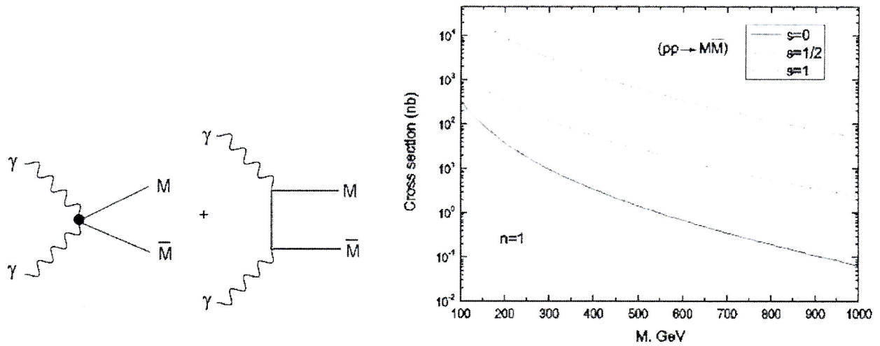
Fig. 4 The two-photon production of monopole-antimonopole pairs at the LHC (left). Cross sections of the process for monopoles of different spin (right)
