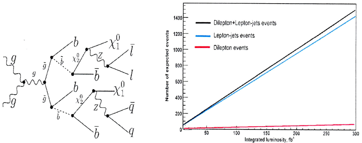
Fig. 5 The "lepton+jets" channel of two gluino decay (left). Number of expected "lepton+jets" (blue line), "dilepton" (red line) and their sum (black line) events at different integrated luminosity with m_{1/2} = 180 GeV (right).
