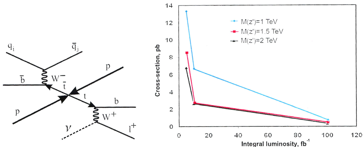
Fig. 3. Lepton+jets channel of the top-anti-top pair decay (left). The 5-sigma confidence level for observation of the tt -resonance (right).
