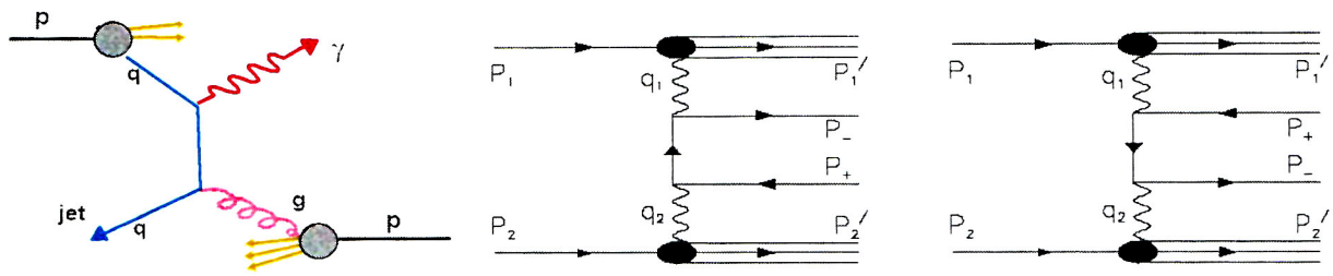
Fig. 6. Determination of gluon distribution in the proton by means of "gamma/Z+jet" events (left). Two-photon Drell-Yan process (right).
