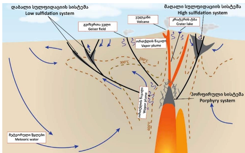
Fig. 1. Model for ore-forming systems of island arcs (Thomsen, 2015).
