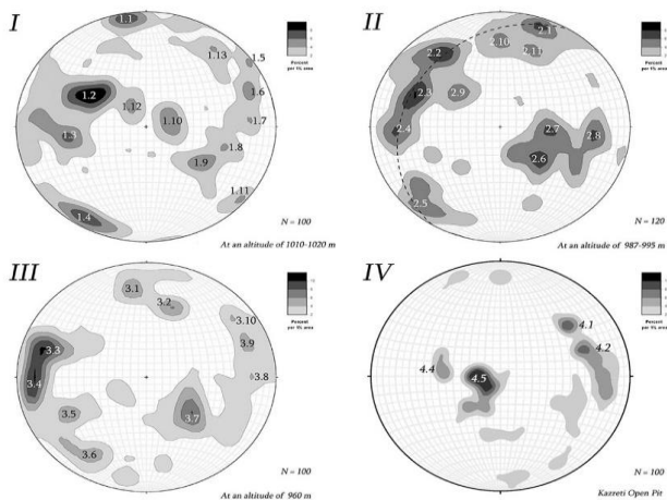
Fig. 1. The lower hemisphere equal-area Schmidt projection of contoured poles to ore veinlets at the Mushevani-2 (I, II, III) and Kazreti (IV) deposits.
