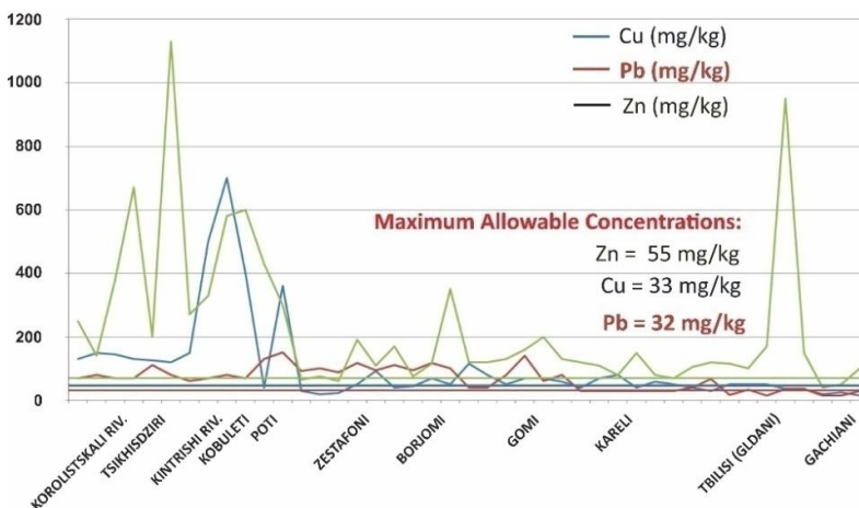
Fig. 1. Copper, Lead and Zinc Contents in Soils along Highways in the Regions of Georgia
